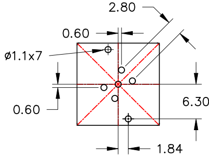
P.C. MOUNTING
