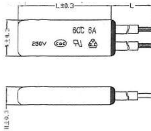
铁壳 Metal case
